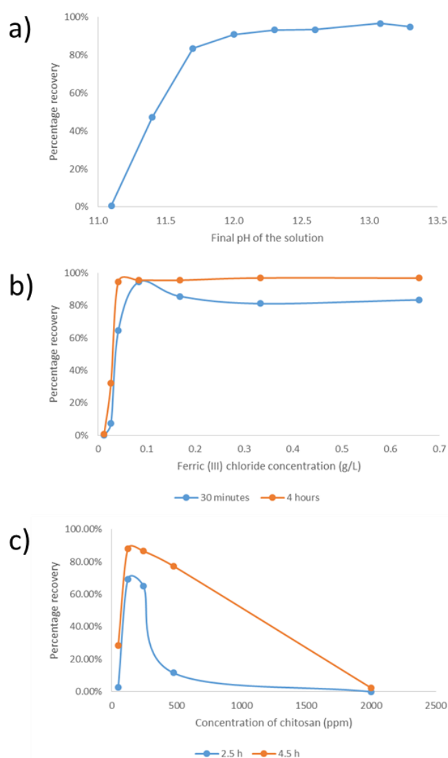
Figure 2. Harvesting efficiency: (a) Sodium hydroxide, (b) ferric chloride, (c) chitosan.
