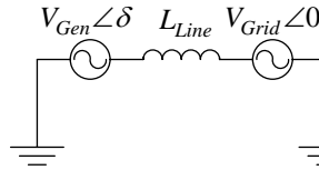
Fig. 1. A simplified model of the grid-connected synchronous machine.
