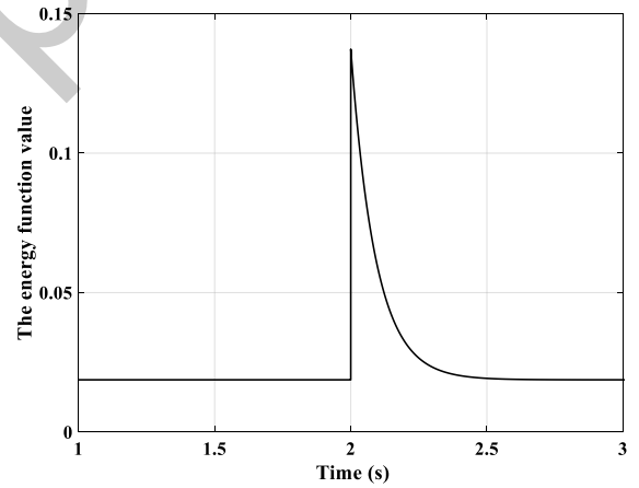
Fig. 8. The energy function value of the grid-connected VSC when the active power reference is changed at t = 2 s.
