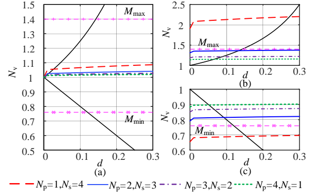
Fig. 17. N_v curve of HMDCSST with different N_p and N_s : (a) at the rated values of V_h and V_l , (b) at 1.05V_h and 0.95V_l and (c) at 0.95V_h and 1.05V_l .
