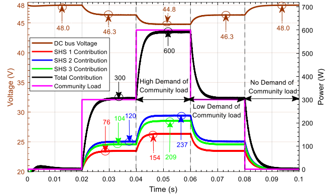
Fig. 6. DC bus voltage V^{DC} profile (left Y-axis) and individual power contributions of various SHS ( P_1^{CL} , P_2^{CL} , and P_3^{CL} ) (right Y-axis) at varying communal load demand in case 3 (simulation results).
