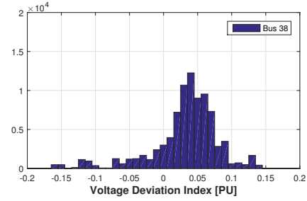
(b) Bus-38 Histogram of Voltage Deviation Index at Secondary Side of Transformer in Excessive Demand Scenario
