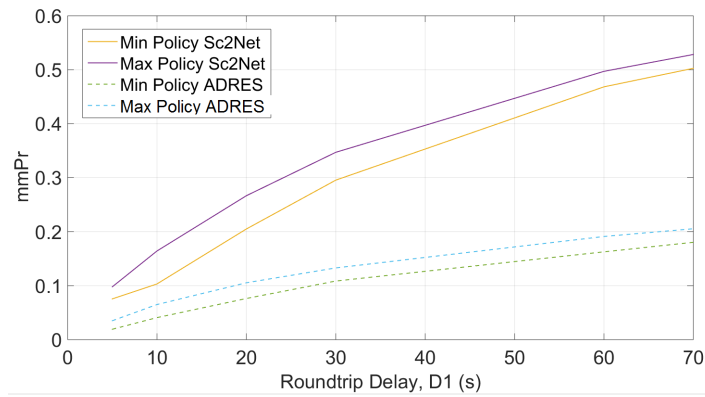
Fig. D.6: Parametric comparison impact of delay on min and max mmPrs for Sc2Net Grid and ADRES Grid
