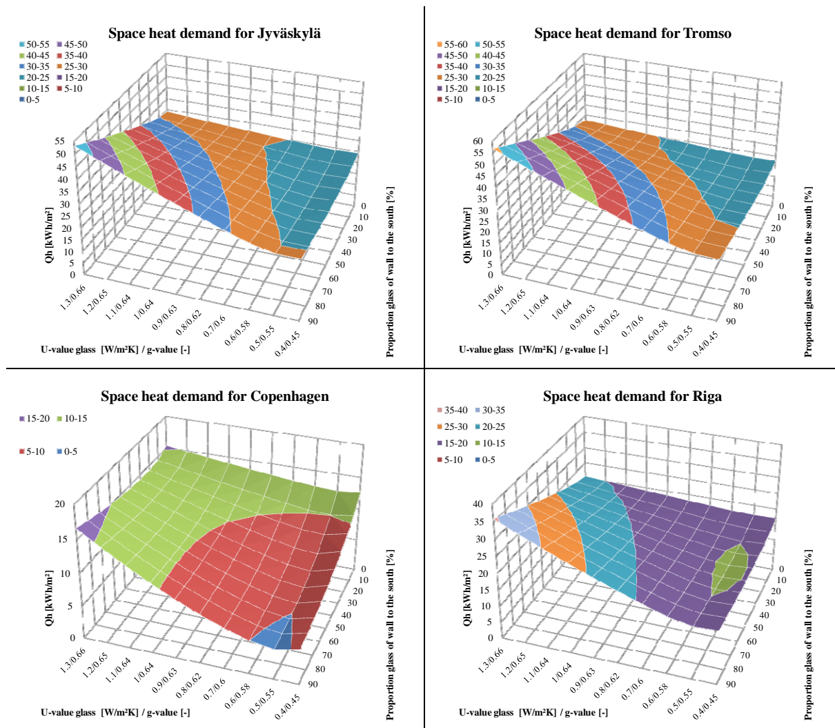
Figure 50. Space heating demand of the single family house (kWh/m 2 ) as a function window g- and U-values (left horizontal axis) and the ratio of the window area to façade area (right horizontal axis). South oriented windows are studied. Fixed window size to every other orientation: N=1%, E=6% and W=6%.
