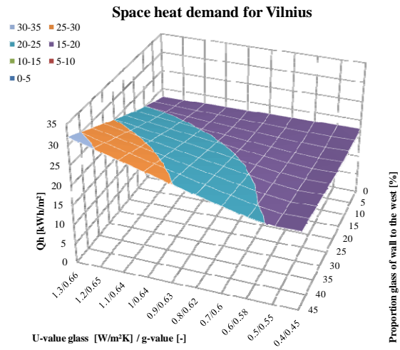
Figure 74. Effect of different window U-values (linked with the g-values) and different glass proportions on the given façade on the space heating demand in Vilnius. No windows to other directions..
