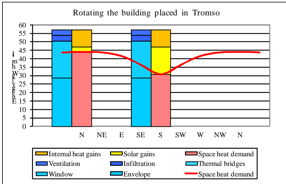
Figure 25. Energy balance of a very low energy house situated in Tromsø, calculated for every 45°. The red line is the resulting space heating demand.
