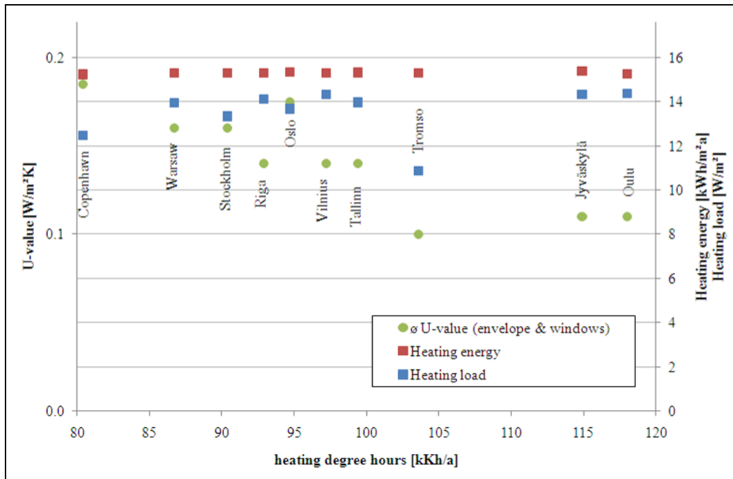
Figure 47. Comparison of the single family house in the different climates. The heat space demand is kept constant and the envelope U-values are varied. U-value is an area weighted mean value of windows and opaque parts.
