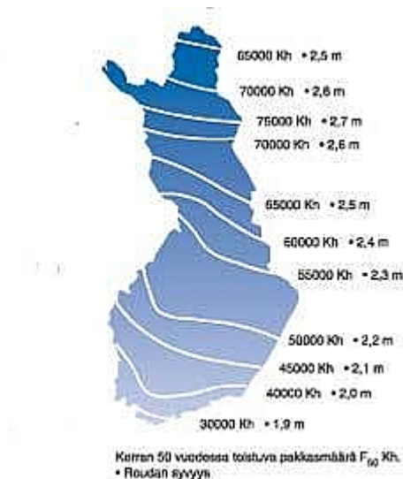
Figure 40: The dimensioning frost free depths for unheated buildings in Finland. Also dimensioning heating degree hours [Kh] are given. F_{50} gives the probability for these degree hours once in 50 years. [15]
