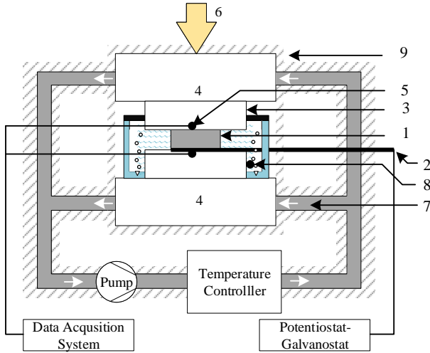
Fig. 7. Schematic of the calorimeter: (1) electrochemical cell under test, (2) current collectors, (3) heat-flux sensor, (4) cold plate, (5) thermocouples, (6) force sensor 0–200 kg \cdot cm^{-2} , (7) cooling fluid, (8) electrolyte bath bubbled with nitrogen, and (9) thermal insulation. [66].
