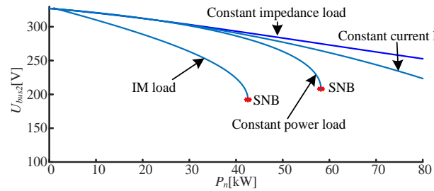
Fig. 10. Equilibrium solution manifold on the P_0 - U_{bus2} plane for load increasing. SNB is saddle-node bifurcation detected in the curve of IM load and constant-power load.
