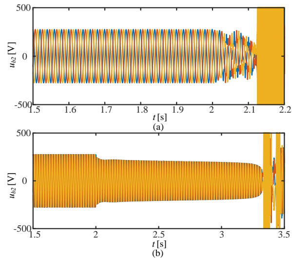
Fig. 19. The phase voltage at bus 2 with 50kW ZIP load. (a) The virtual inductance of is switched from 4mH to 6mH at 2s. (b) The nominal voltage of droop controller is switched from 330V to 300V at 2s.
