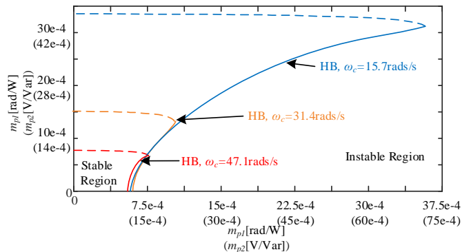
Fig. 7. Hopf bifurcation boundaries for MG with different cut-off frequency.
