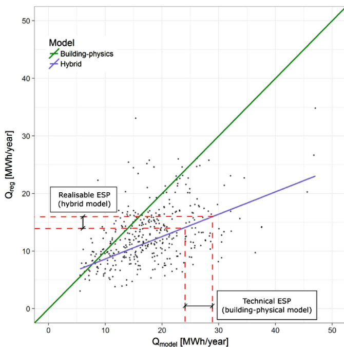
Fig. 7. Conceptual illustration of the difference between the technical- and the realisable energy-saving potential (ESP) in a subset of the considered sample.
