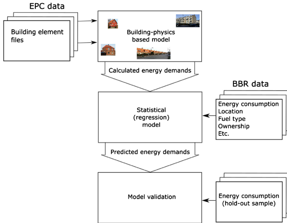
Fig. 3. Hybrid model flowchart. The building-physics based model, which can be used for studying effects improving the energy efficiency of a building, was used as input in the statistical (MLR) model.
