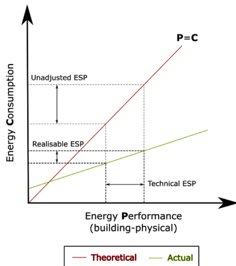
Fig. 1. Relationship between the building-physical energy performance (P) and the related energy use (C) of a building. Conceptual illustration (adapted from [17,20]).
