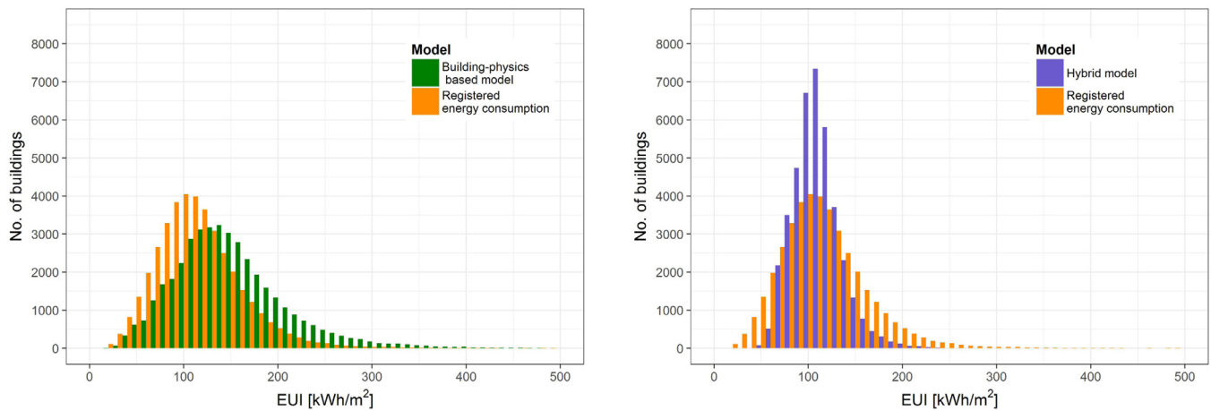
Fig. 5. Heat demands estimated with the building-physical model (left) and the hybrid model (right) respectively, both compared with the registered energy use.
