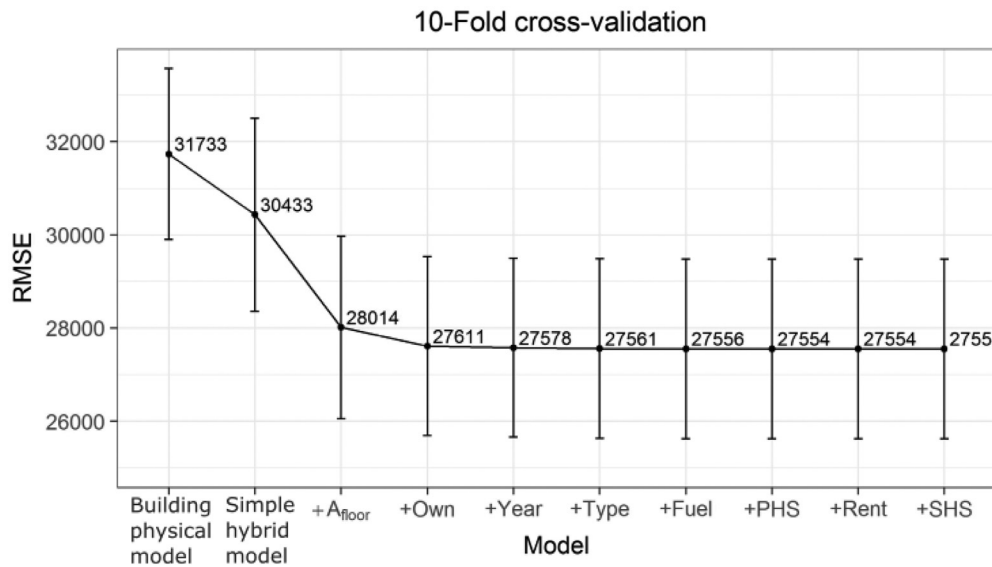
Fig. 4. Model selection based on the marginal improvement in RMSE of each model calculated using 10-fold cross-validation. The error-bars illustrate the standard-error of the RMSE in each model.
