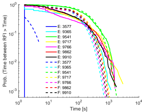
Fig. 7: Empirical RFI inter-arrival time (solid lines) and fitted exponential distributions (dashed lines) for selected interference sources from data obtained on the roof top. Parameter of fitted distributions are presented in Tab. II.
