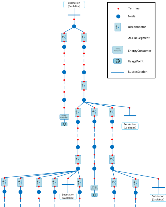
Fig. 2: Subset of LV grid topology extracted by GT-HE out of the complete CIM-XML based topology file.
