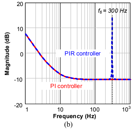
Fig. 3. Amplitude and frequency characteristic curve. (a) LCL filter characteristic from converter/grid voltage to filter capacitor voltage and current. (b) PI and PIR controller.
