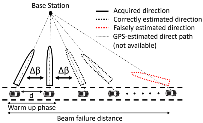
Fig. 1. Beam tracking exploiting only acquired signal direction
