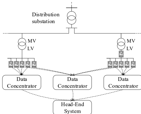
Figure 1: Typical AMI system architecture.
