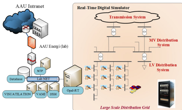
Figure 6: Laboratory setup system architecture deployed for RemoteGRID project activities.
