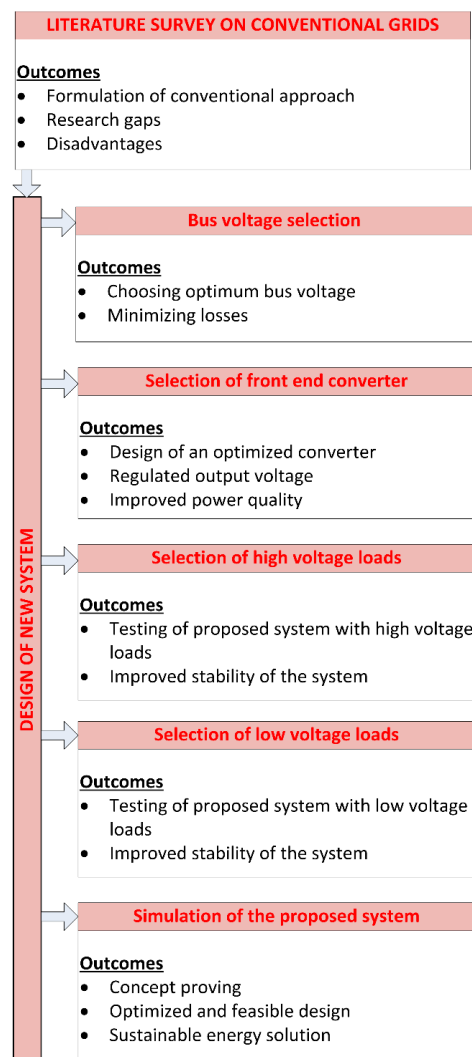
Figure 1. Methodology outline.
