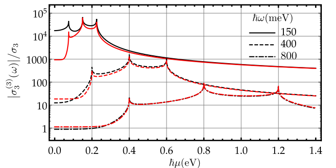
FIG. 2. THG conductivity in gapped ( E_g = 250 \text{ meV} , black) and gapless (red) graphene at photon energies \hbar\omega = \{150, 400, 800\} \text{ meV} .
