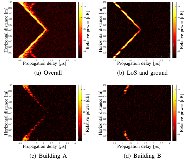
Fig. 6: Simulated CPDPs.
