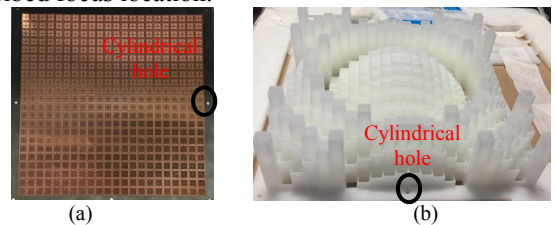
Fig. 4. Prototypes of the proposed high-gain and filtering transmitarray antenna components. (a). SIW cavity bandpass filter. (b). APDSP-based dielectric lens.
