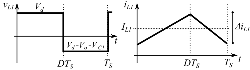
Fig. 2: Voltage and current waveforms of the inductor L_1 .
