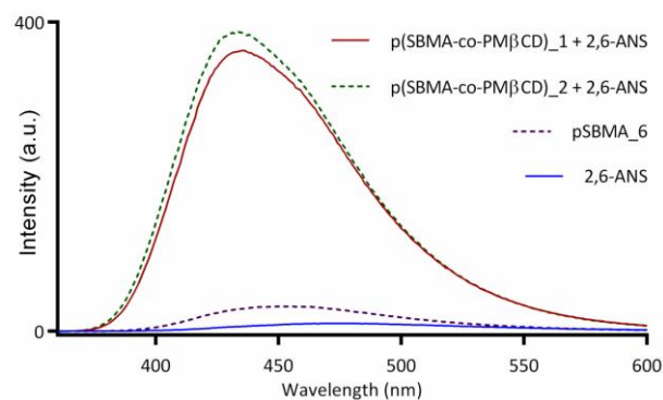
Figure 5 – Fluorescence emission spectra of 2,6-ANS ( \sim 150 \mu M) with and without pSBMA_6 (10 mg mL ^{-1} ), p(SBMA-co-PM \beta CD)_1 (10 mg mL ^{-1} ) and 2 (5 mg mL ^{-1} ).
