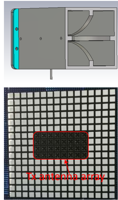
Figure 2. CST simulation model of the Tx antenna element (top) and a photo of the Tx antenna array (below).
