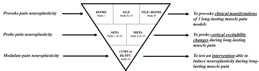
Fig. 1 Dissertation outline.
