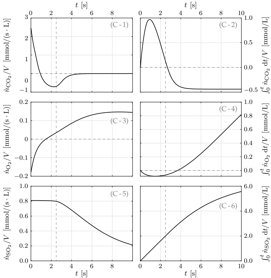
Figure 3.13: The mass transfer rates of CO 2 (g), O 2 (g), and SO 2 (g) per unit volume in the left column, and the cumulative temporal integral of the rates in the right column. The vertical dashed lines are indicating A_T = 0 .
