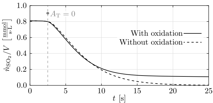
Figure 3.14: The effect of oxidation on the absorption rate of SO 2 .
