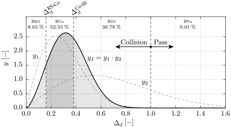
Figure 4.40: The probability density function for both parcels, y_1 and y_2 , along with the joint probability, y_J = y_1 \cdot y_2 , as a function of \Delta_d . \Delta_d^{\text{RS-Co}} and \Delta_d^{\text{Co-SS}} are interpolated from Figure 4.37 at We = 44 for the given example.
