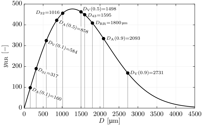
Figure 4.11: A Rosin-Rammler distribution with various characterizing metrics overlaid, where all numbers have units of \mu\text{m} .
