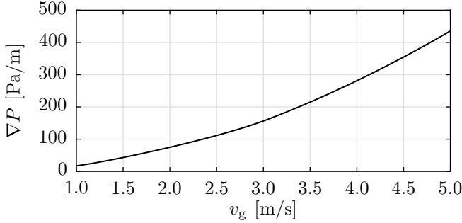
Figure 4.46: The specific pressure loss of the demister [Munters (97)].
