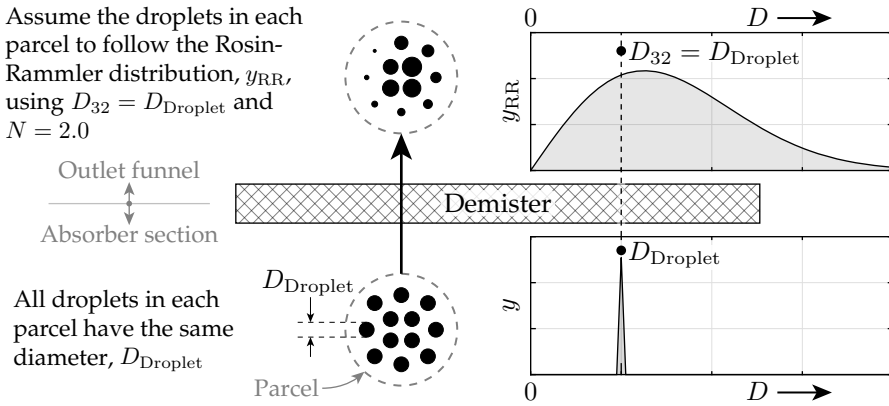
Figure 4.43: When a parcel hits the demister, it is assumed that the droplets within each parcel follow the Rosin-Rammler distribution, y_{\text{RR}} , which allows for analytical integration of the demister efficiency.
