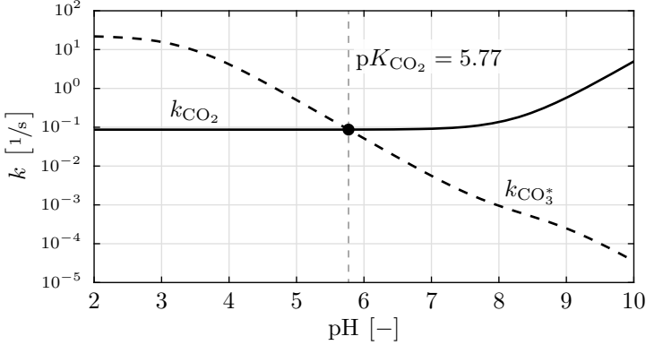
Figure 3.7: The overall rate constants in (3.34) as functions of pH.
