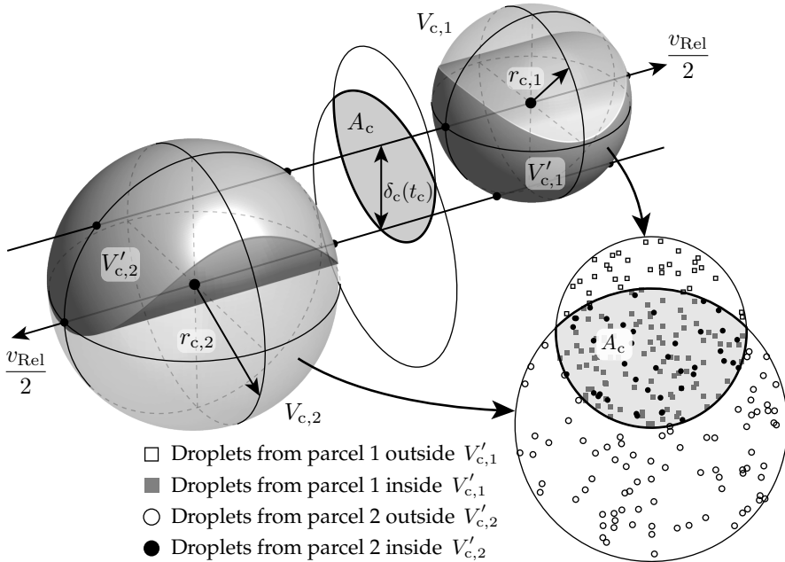
Figure 4.33: An illustration of the swept intersecting volumes of two collision spheres. V_c are the collision spheres, and V'_c are the swept overlapping volumes of the collision spheres. A_c is the intersecting area. Notice that the droplets inside the parcels are omitted in this illustration for visualization purposes.
