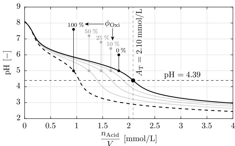
Figure 3.8: Titration curves for five different values for \phi_{\text{Oxi}} .
