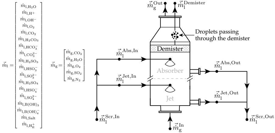
Figure 7.6: The flows going in and out of the scrubber. The mass flow vectors \vec{m}_l and \vec{m}_g are shown to the left, where all components in the two phases are shown.
