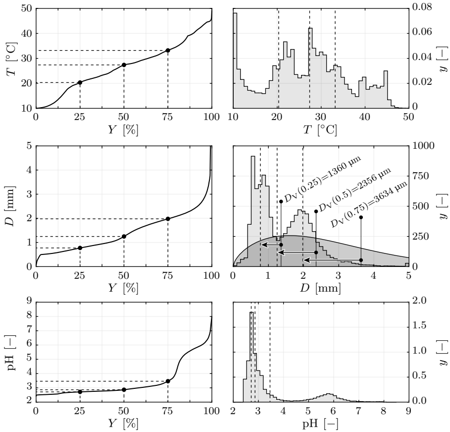
Figure 11.5: The distributions of T , D , and \text{pH} for the discrete phase. The left and right figures are showing the cumulative, Y , and probability, y , density functions respectively. The dashed lines are indicating the 25, 50, and 75 % fractiles.
