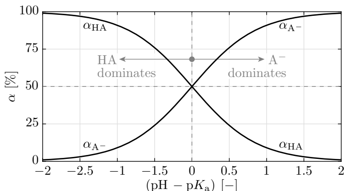
Figure 3.4: \alpha_{\text{HA}} and \alpha_{\text{A}^-} as a function of (\text{pH} - \text{p}K_a) . When \text{pH} = \text{p}K_a , the concentrations of [\text{HA}] = [\text{A}^-] , where \alpha_{\text{HA}} = \alpha_{\text{A}^-} = 50\% .
