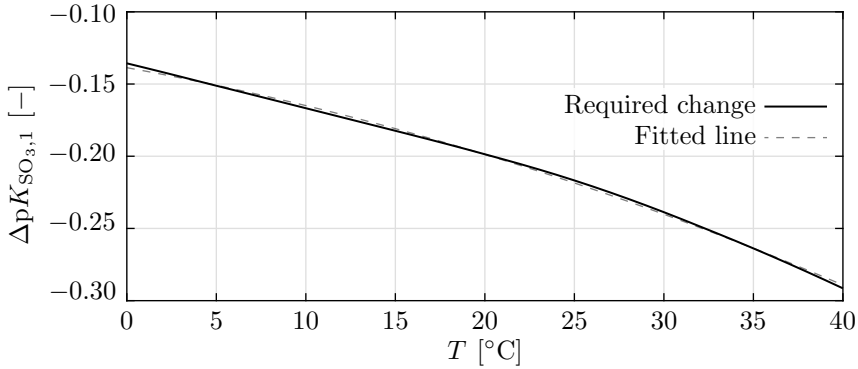
Figure 3.18: The required value of \Delta pK_{\text{SO}_3,1} to meet the average absorption rate of the full chemistry model.
