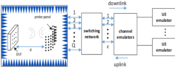
Fig. 1. Illustration of sectored MPAC based mmWave OTA testing system.
