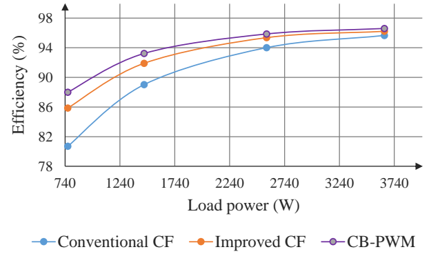
Fig. 8. Measured efficiency of the three-phase VSC using the three controlling algorithms, feeding a non-linear load.
