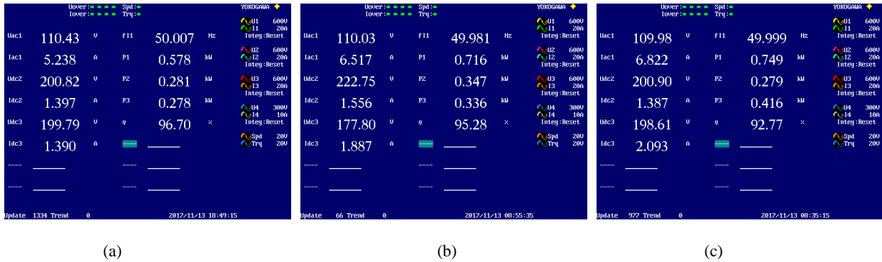
Fig. 14. The efficiency test results of the proposed converter when V_g = 110 V, E = 400 V. (a) In the balanced-load mode ( R_1 = 144 \Omega , R_2 = 144 \Omega ). (b) In the unbalanced-load mode without regulation ( R_1 = 144 \Omega , R_2 = 94 \Omega ). (c) In the unbalanced-load mode with regulation ( R_1 = 144 \Omega , R_2 = 94 \Omega ).
