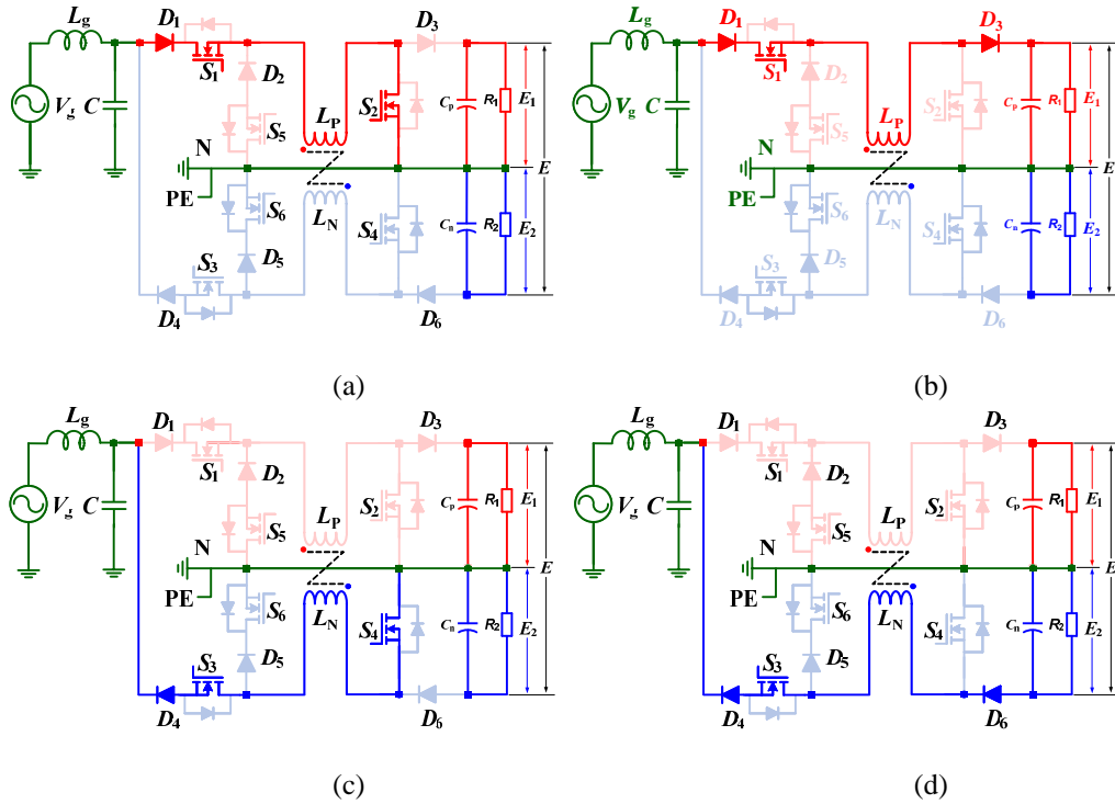
Fig. 4. Equivalent circuits in the ‘‘Boost’’ state: (a) Energy storing in the positive half of line period, (b) Energy releasing Energy storing in the positive half of line period, (c) Energy storing in the negative half of line period, (d) Energy releasing in the negative half of line period.
