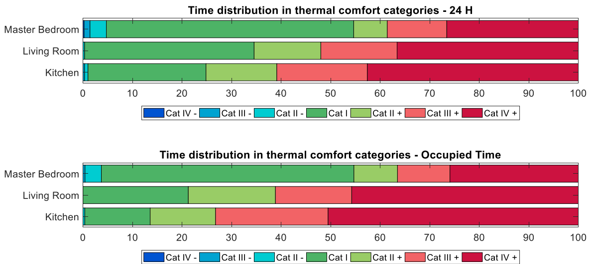
Figure 10: Percentage of time in each Category for temperature during 3 months period time (June, July, August)
