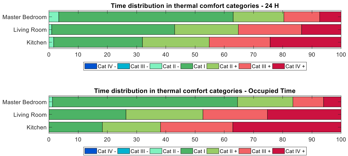
Figure 7: Percentage of time in each Category for temperature during May
