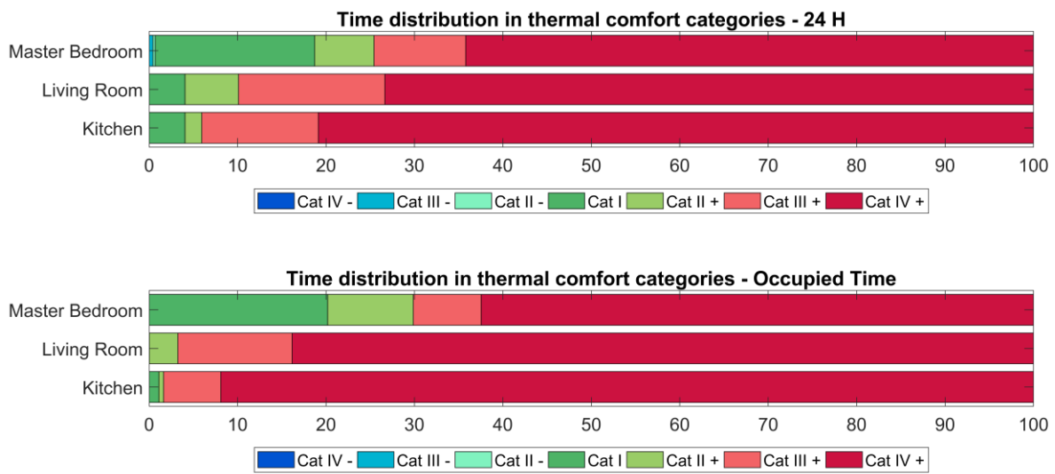
Figure 9: Percentage of time in each Category for temperature during July
