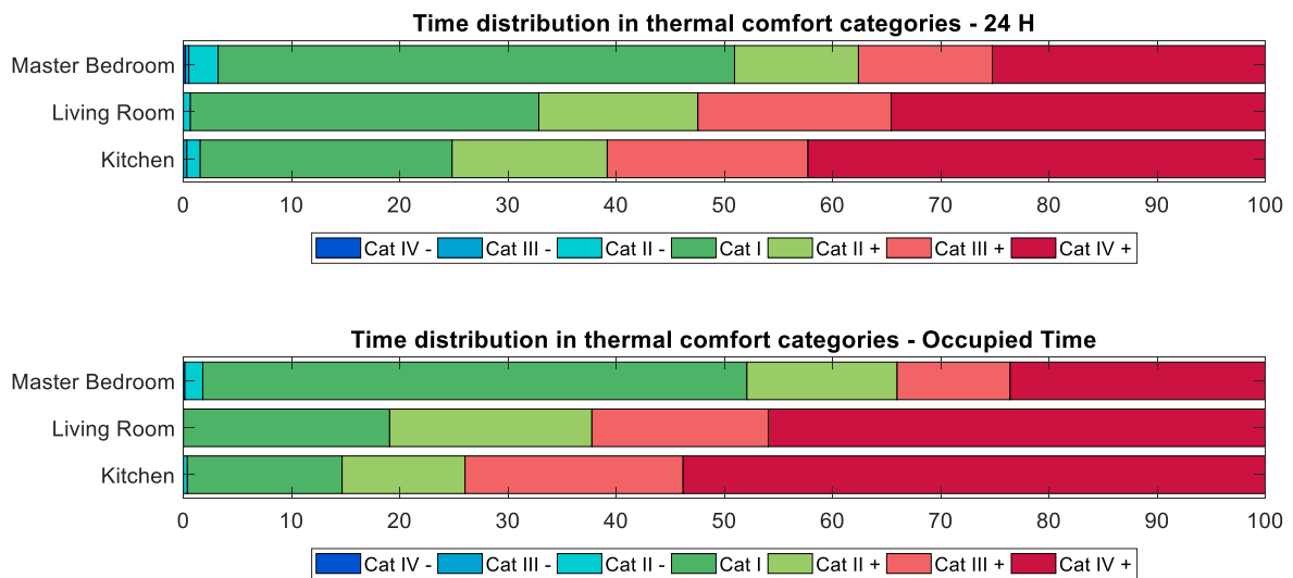
Figure 10: Percentage of time in each Category for temperature during 3 months period time (May, June, July)
