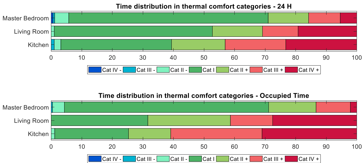
Figure 8: Percentage of time in each Category for temperature during June
