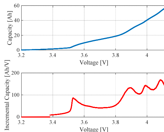
Fig. 1. Capacity (top) and IC (bottom) as a function of the battery voltage.
