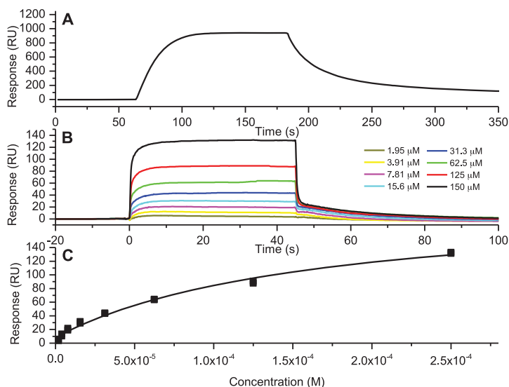
FIGURE 2. A and B , sensorgrams showing the interaction of Congo Red at 10 \mu\text{M} ( A ) and ThT at concentrations of 1.95–150 \mu\text{M} ( B ) with FapC fibrils. C , dose-response curve for the interaction between ThT and FapC fibrils. RU , response units.
