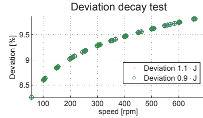
Fig. 14: Deviation of losses calculation with changing J .
