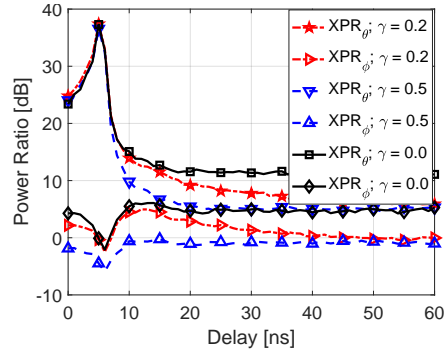
Fig. 8: Effects of mixing parameter on power ratio.
