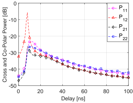
Fig. 5: Co and Cross-Polar Power for \pm 45^\circ MIMO channel. Receiver at Location II.
