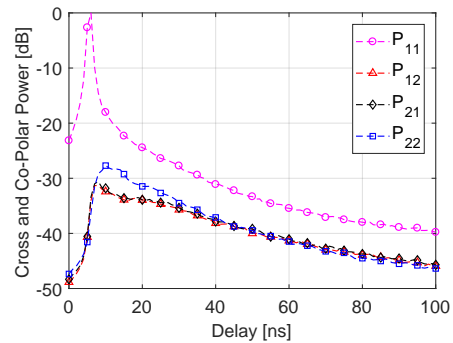
Fig. 3: PDP for 0/90^\circ MIMO channel. Receiver at Location I.
