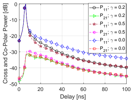
Fig. 7: Effects of mixing parameter on PDP.
