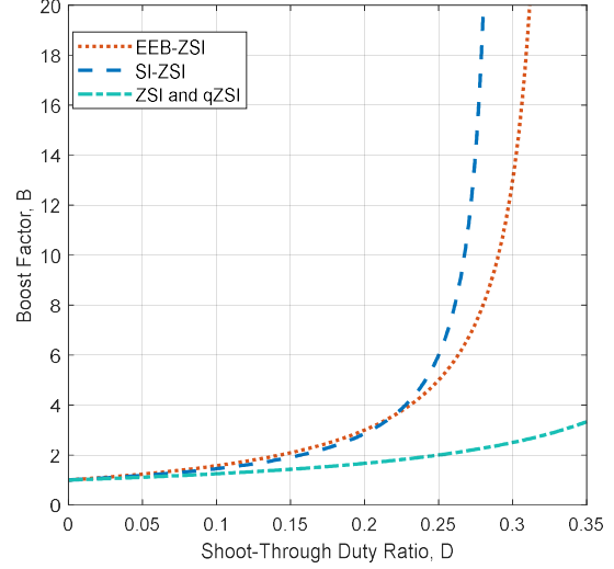
Fig. 5. Boost factor comparison of three Z-source inverters (i.e., the ZSI/qZSI, SI-ZSI, and EEB-ZSI).
