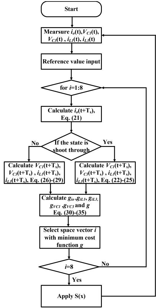
Fig. 7. Flow chart of the proposed MPC for the EEB-ZSI.
