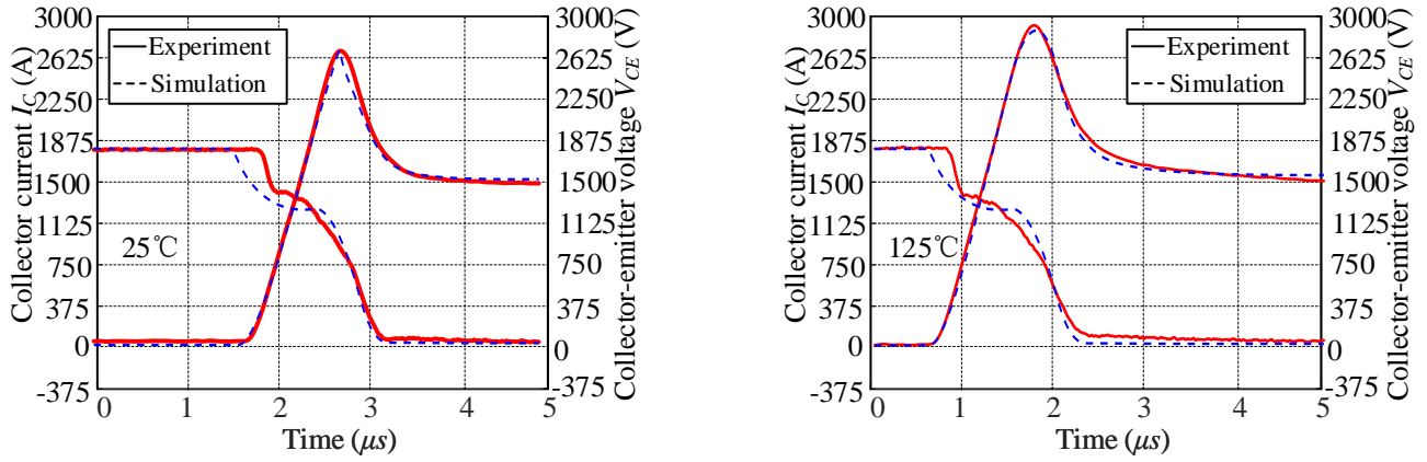
Fig. 7. Comparison between experiment and simulation on turn-on transient at different temperature: (a) V_{DC}=1800V , I_C=1500A , T=25^\circ C ; (b) V_{DC}=1800V , I_C=1500A , T=125^\circ C .
