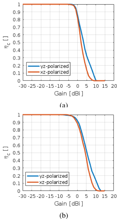
Figure 10. Coverage efficiency of phased antenna array in (a) configuration 1 and (b) configuration 2.
