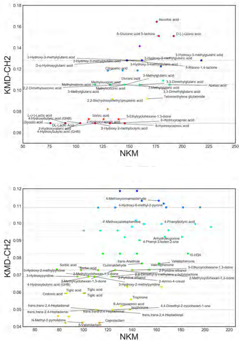
Figure 8: Kendrick plots for the molecular species constituting the core composition of the samples (constant amounts in all the samples regardless of process conditions) with a area threshold of 10^7 for negative (top) and positive (bottom) ESI ionization.
