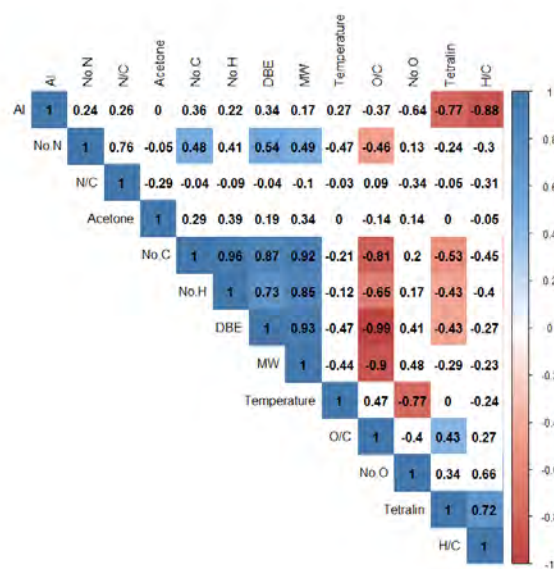
Figure 4: Spearman matrix showing the direction and strength of the linear association between process conditions and an average species' properties. Statistically significant ( p -value <0.005 ) direction of the association are outlined in red (negative) and blue (positive) with the magnitude of the correlation coefficients indicating the strength of the association.
