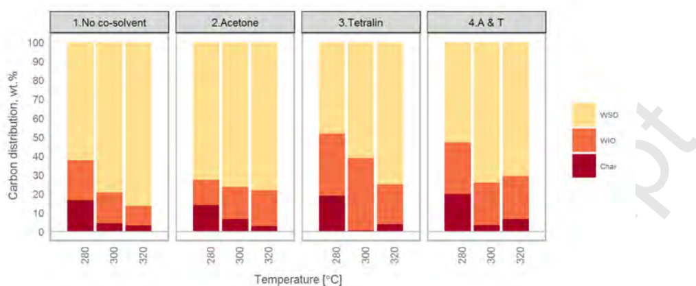
Figure 1: Distribution of carbon in the product fractions from different runs.
