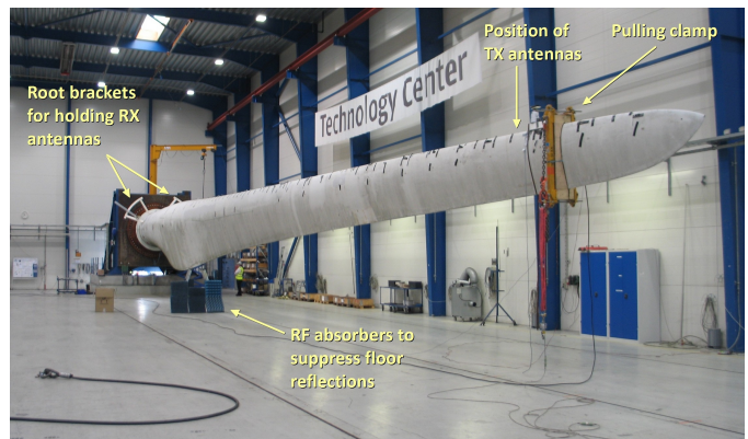
Fig. 2. Setup of Experiment 1 – the dynamic pull test. The blade can be seen from its downwind side. The cable that will be attached to the pulling clamp and perform the bending is visible lying on the floor, bottom left.
