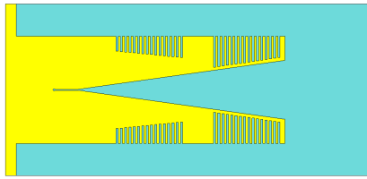
Fig. 19. The corrugated Vivaldi antenna used as a TX antenna (left) and the UWB dipole used as an RX probe (right).
