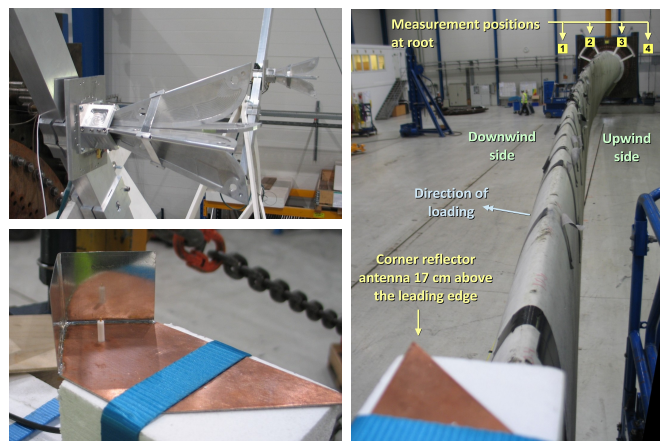
Fig. 3. Top left: Dual-polarized quad-ridged horn antennas used as the RX antennas at the root; Bottom left: Corner reflector antenna used as the TX antenna at the blade tip; Right: View from the tip towards the root when the blade is the prebend state. Positions of the RX antennas at the root are denoted. The corner reflector antenna sitting on a 17 cm high styrofoam block can partially be seen in the front.
