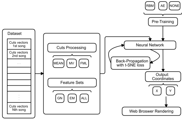
Figure 1: Flow chart of the work starting from the dataset storing the stack of cuts representing each song, till the rendering.
