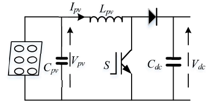
Fig. 2 PV system configuration.
