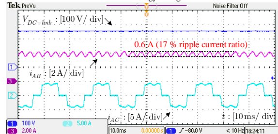
(b) Diode-bridge rectifier with a passive inductor with 0.51 J rated inductive energy storage.
