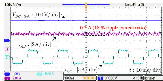
(a) Diode-bridge rectifier with an active inductor with 0.14 J rated inductive energy storage.
