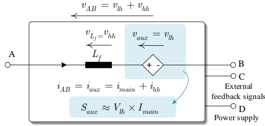
(a) The equivalent diagram of the active inductors proposed in [3-5].
