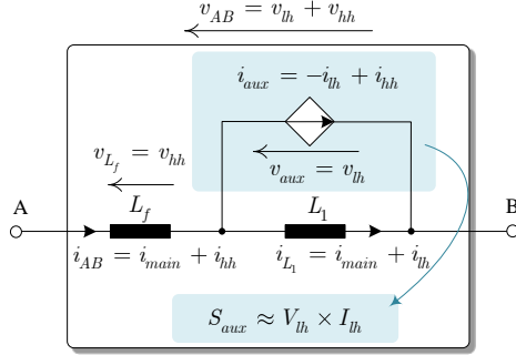
(b) The equivalent diagram of the proposed two-terminal active inductor.
