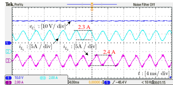
Fig. 8. Experimental waveforms of the active inductor in the case study.
