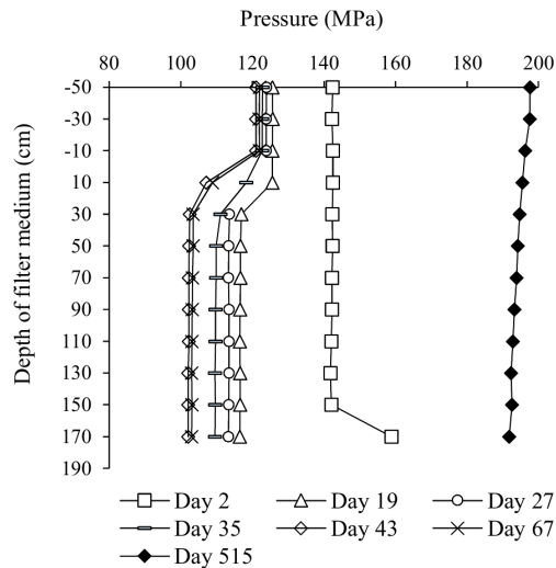
Figure 4. Pressure profile of Filter 1 over time. Measurements were carried out just prior to a backwash, except Day 2.
