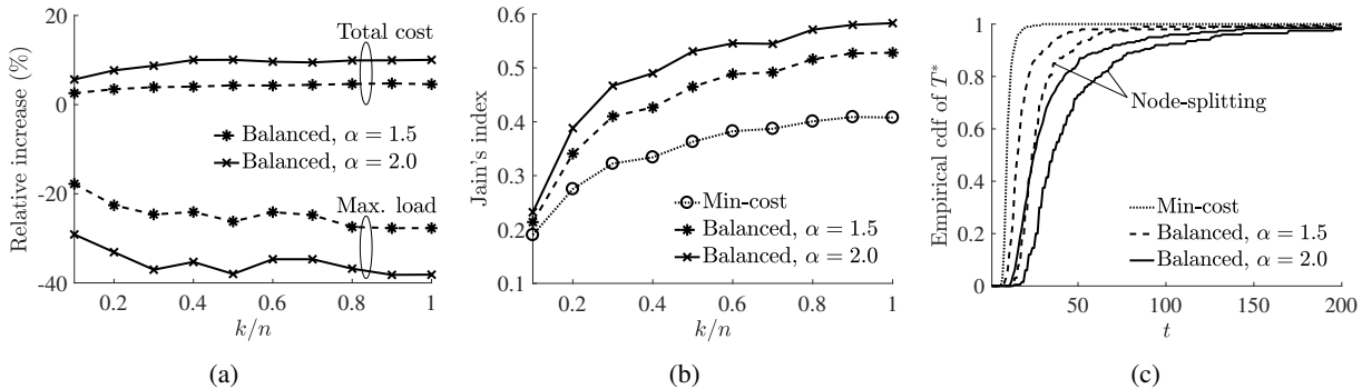
Fig. 1. Simulation results for n = 50 , m = 1 and various fractions k/n of source nodes: (a) Improvement of the total cost and maximum load relative to minimum-cost routing; (b) Jain's fairness index for the node loads; (c) empirical cdf of the minimum number T^* of iterations required for Algorithm 1 to converge when k/n = 0.3 .
