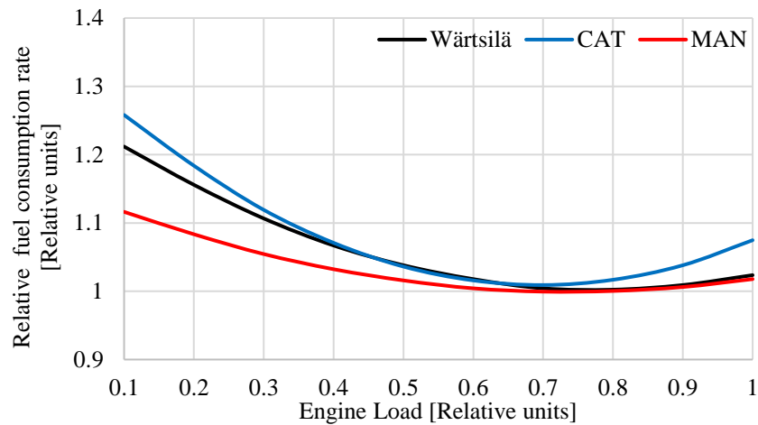
Fig. 1. The relative SFOC based on data of three manufacturers: Wärtsilä, Caterpillar and MAN [43]
