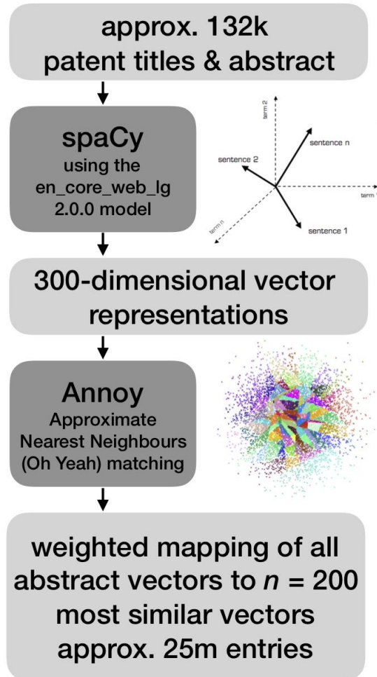
Figure 7: Preprocessing pipeline
