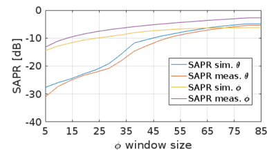
Fig. 8. SAPR of the \theta and \phi polarizations of bi-conical antenna simulated with the phantom and measured with the user.
