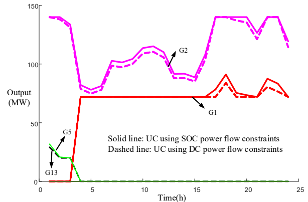
Figure 5 Output Curve of each generator using different UC models
