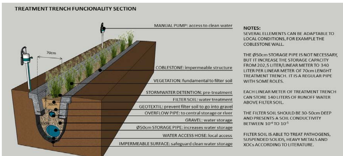
The figure illustrates one possible design of the Treatment Trench and its different components.
