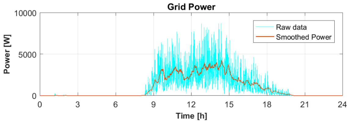
Figure 17: Comparison between the generated power by the hybrid system and the smoothed grid-injected power – summer.
