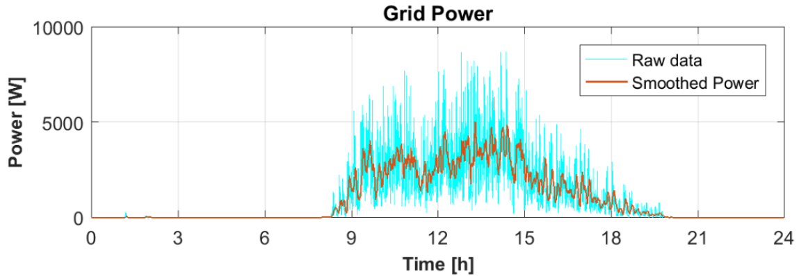
Figure 13: Comparison between the generated power by the hybrid system and the smoothed grid-injected power – summer.
