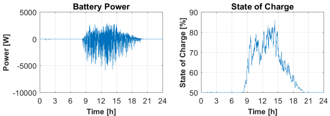
Figure 18: Battery behavior: power (left) and SOC profile (right) – summer.
