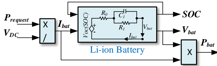
Figure 5: Block diagram of the lithium-ion battery model.
