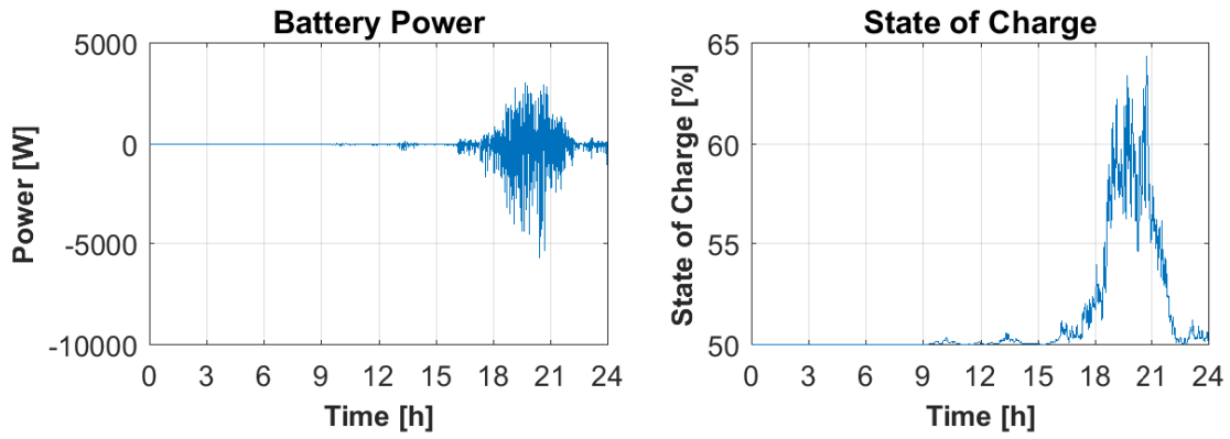
Figure 16: Battery behavior: power (left) and SOC profile (right) – winter.
