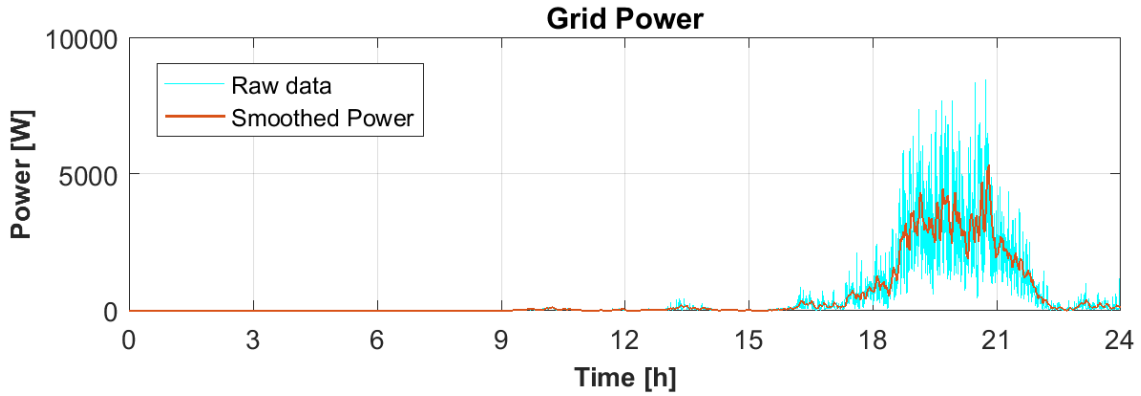
Figure 19: Comparison between the generated power by the hybrid system and the smoothed grid-injected power – winter.
