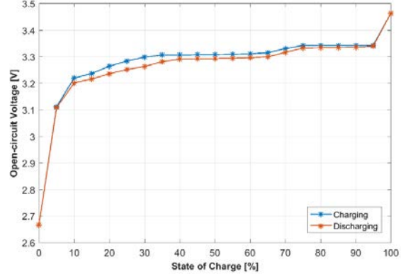
Figure 7: OCV vs SOC characteristic during charging and discharging.
