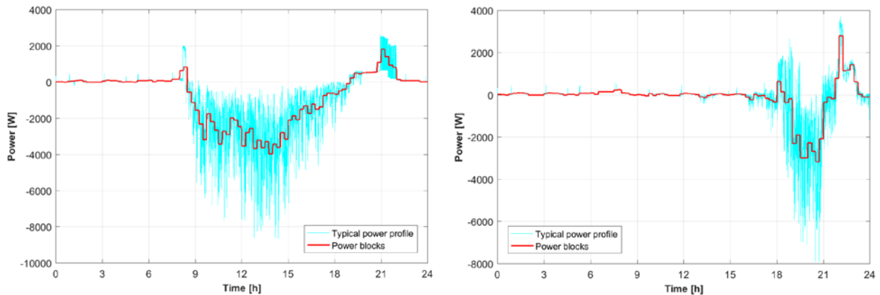
Figure 21: Typical power profile and power blocks for a summer day (left) and a winter day (right).
