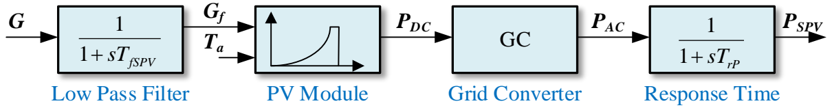
Figure 2: Block diagram of the SPVM.
