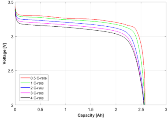
Figure 6: Dependence of the battery discharging capacity on the C-rate.
