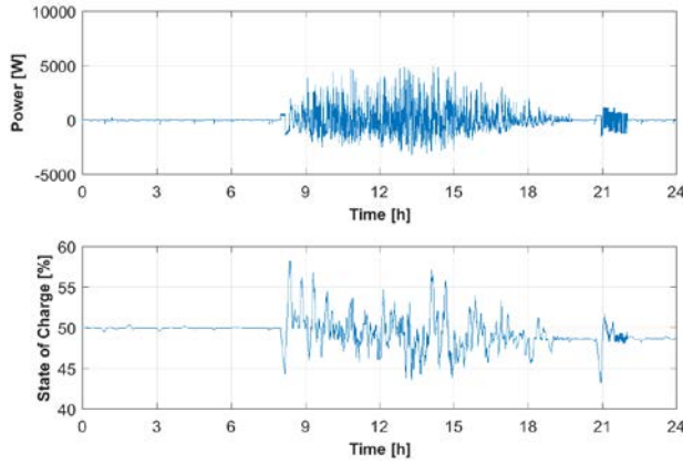
Figure 22: Battery power and SOC during power blocks EMS for a summer day.
