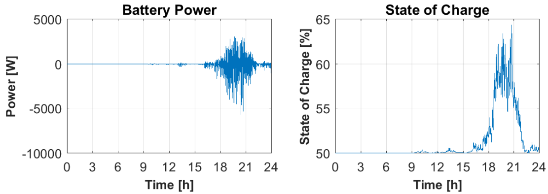
Figure 20: Battery behavior: power (left) and SOC profile (right) – winter.
