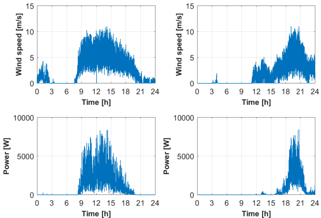
Figure 10: Wind speed (top) and corresponding WT power (bottom) for one summer (left) and one winter day (right).
