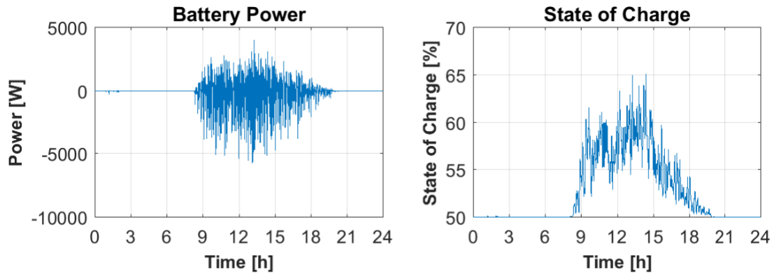
Figure 14: Battery behavior: power (left) and SOC profile (right) – summer.
