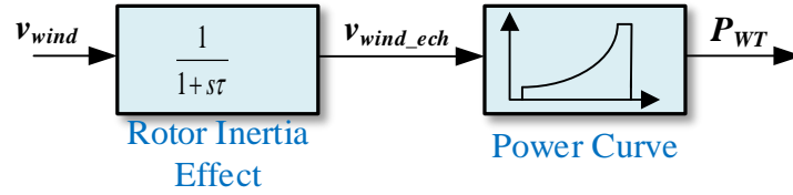
Figure 3: Block diagram of the wind turbine.
