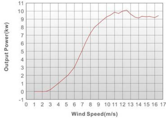
Figure 4: Power curve of the 10 kW WT [14]
