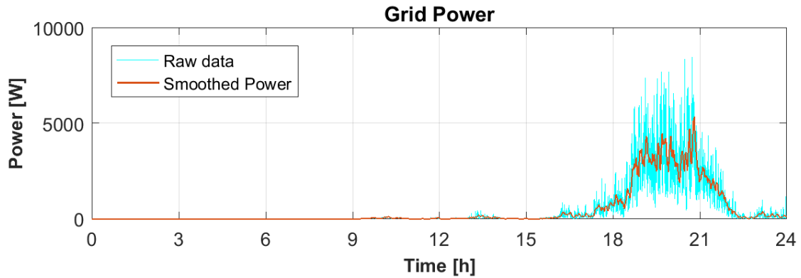
Figure 15: Comparison between the generated power by the hybrid system and the smoothed grid-injected power – winter.
