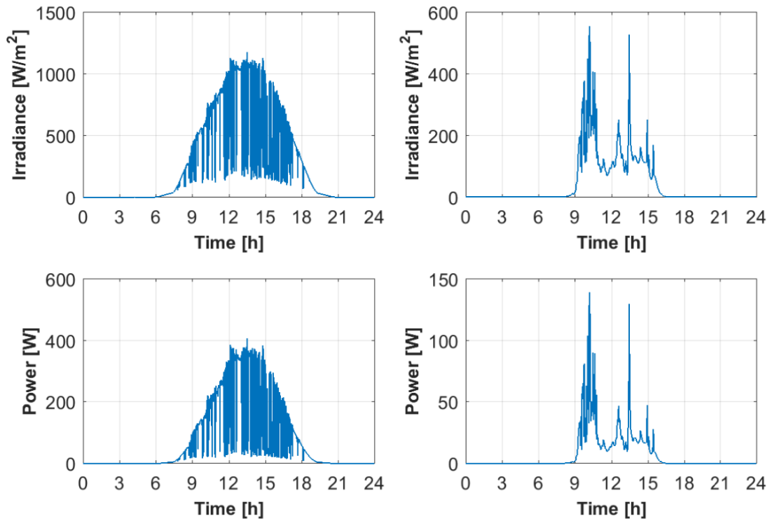
Figure 9: Irradiance (top) and corresponding PV power (bottom) for one summer day (left) and one winter day (right).
