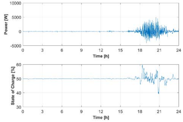
Figure 22: Battery power and SOC during power blocks EMS for a winter day.
