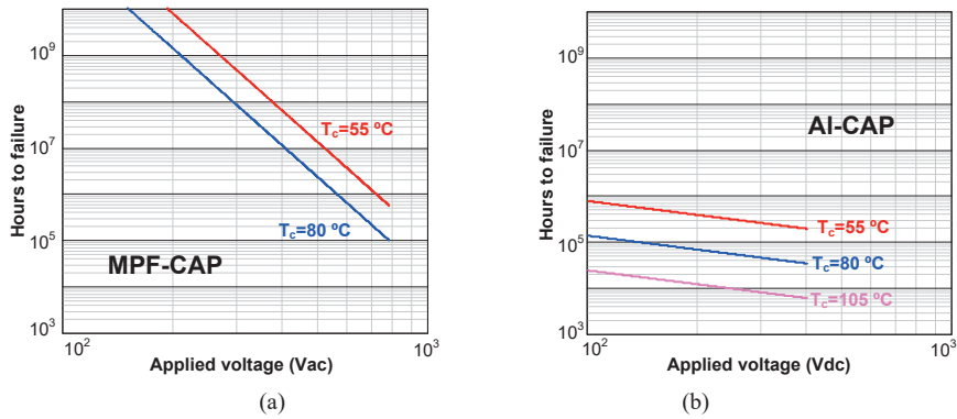
Fig. 5. Hour to failure in respect to various applied voltage and various operational temperature. (a) Metalized polypropylene film capacitor; (b) Aluminum electrolytic capacitor.
