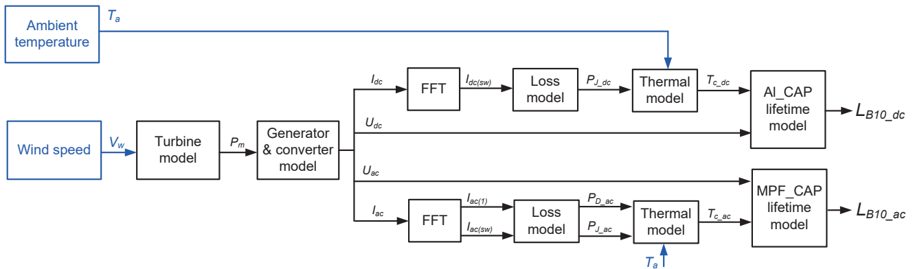
Fig. 4. Flowchart to calculate B_{10} lifetime from mission profile.
