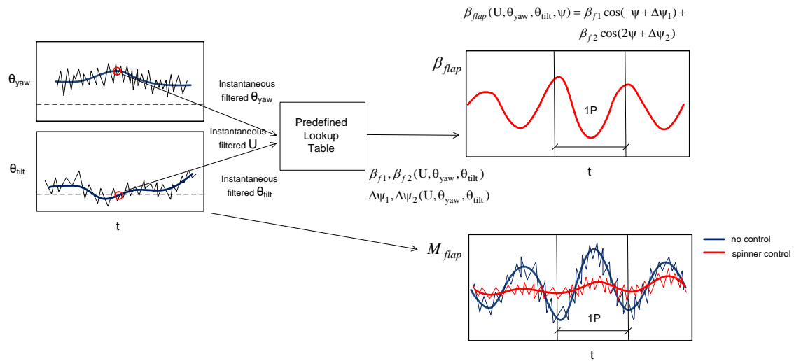
Figure 6-10 IFPC-FF schematic
